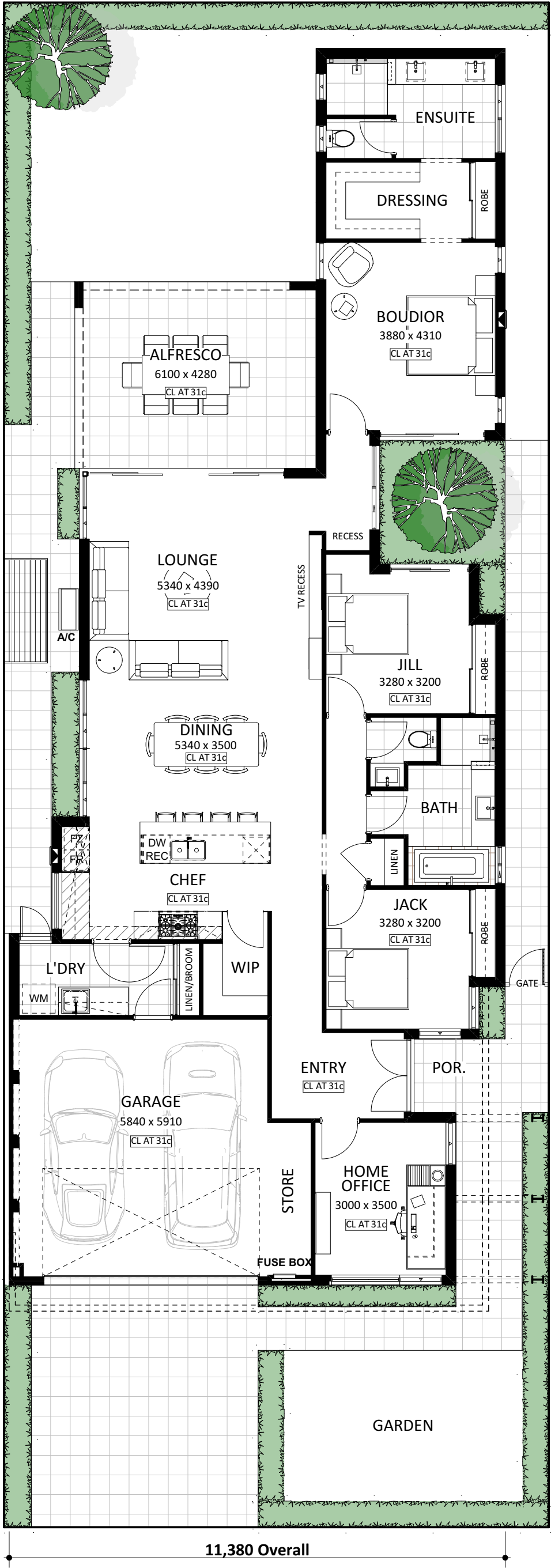
FLOOR PLAN 1:100
