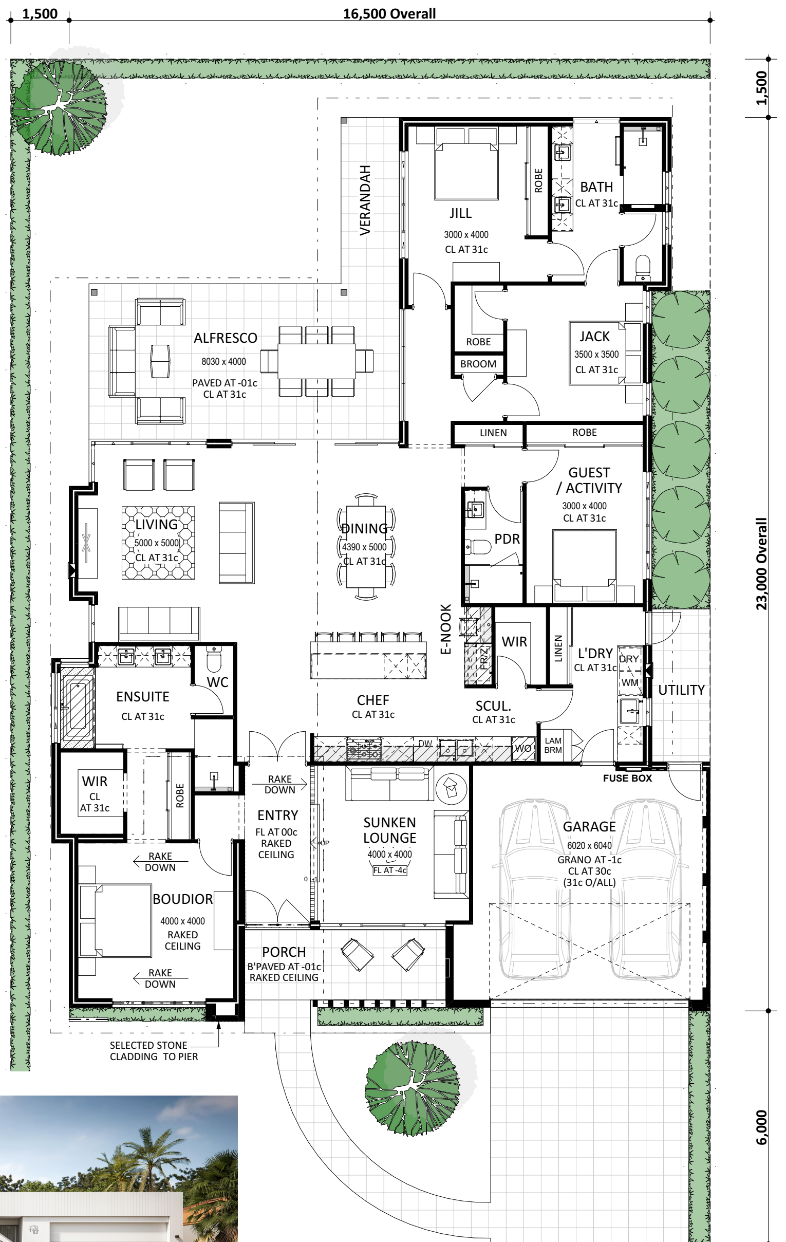
FLOOR PLAN
