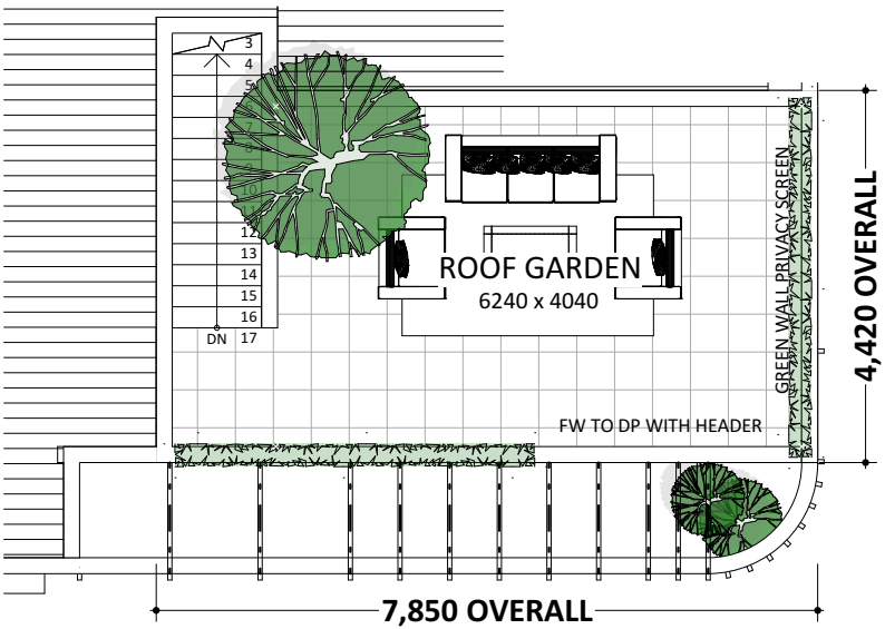
ROOF GARDEN PLAN 1:100
