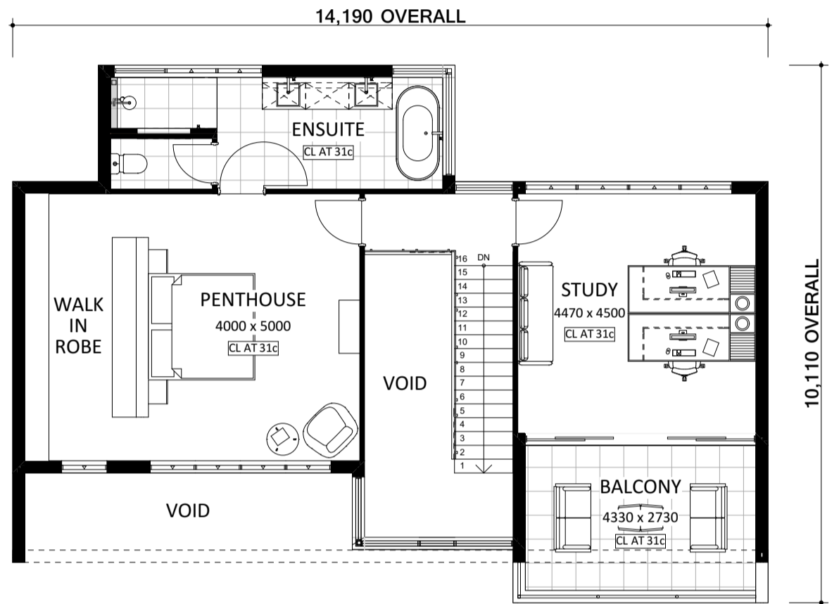
UPPER FLOOR PLAN 1:100
