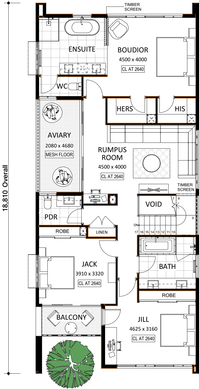
UPPER FLOOR PLAN 1:100
