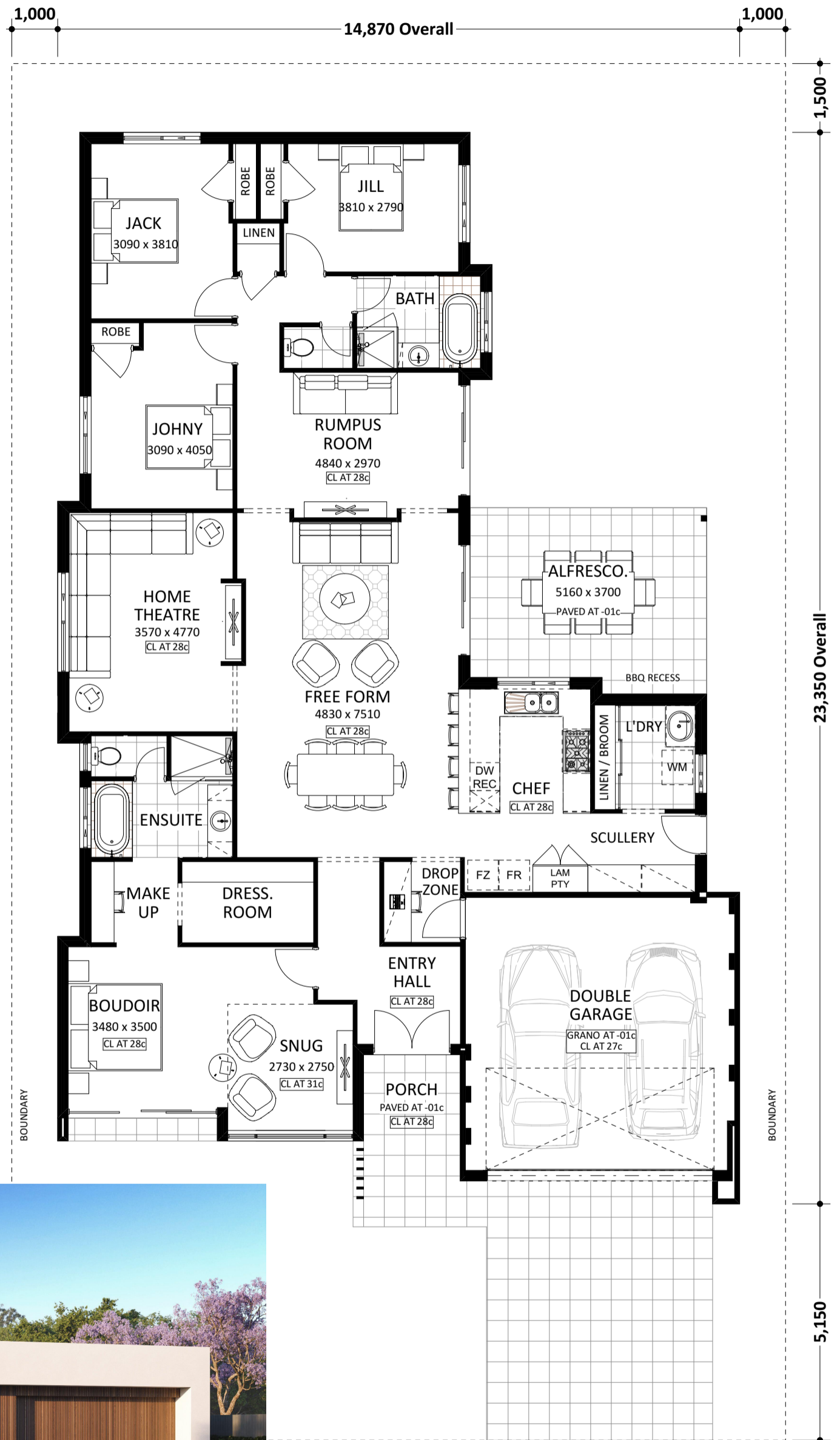
FLOOR PLAN 1:100
