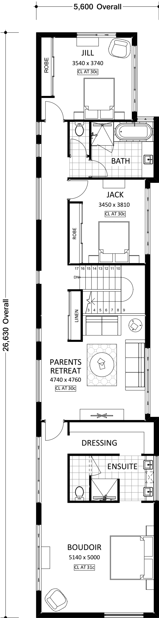
UPPER FLOOR PLAN
