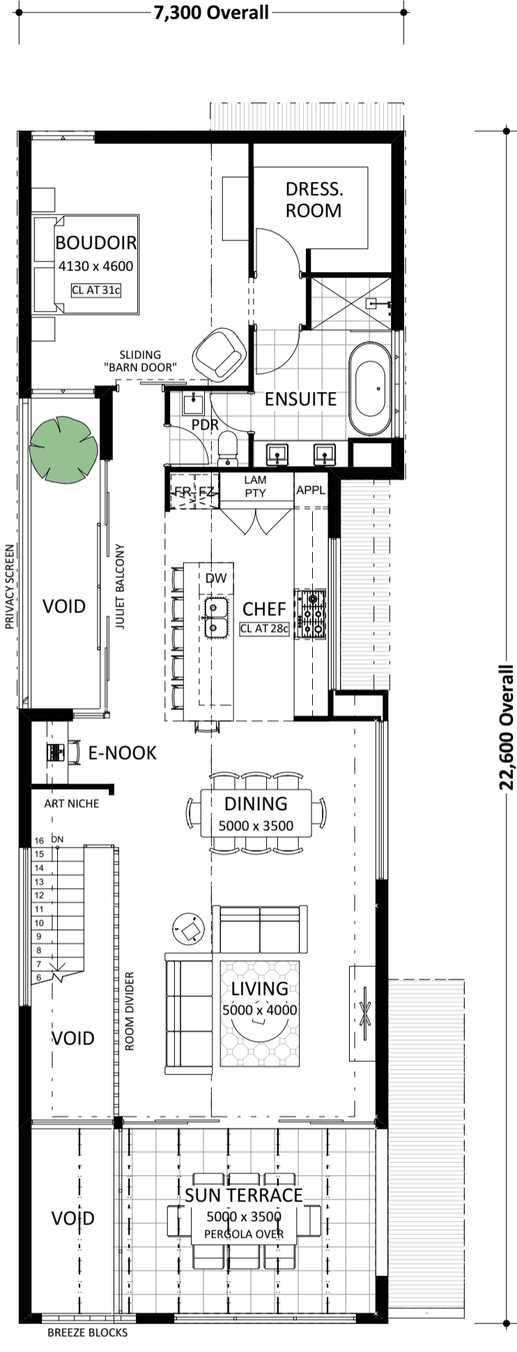
UPPER FLOOR PLAN 1:100
