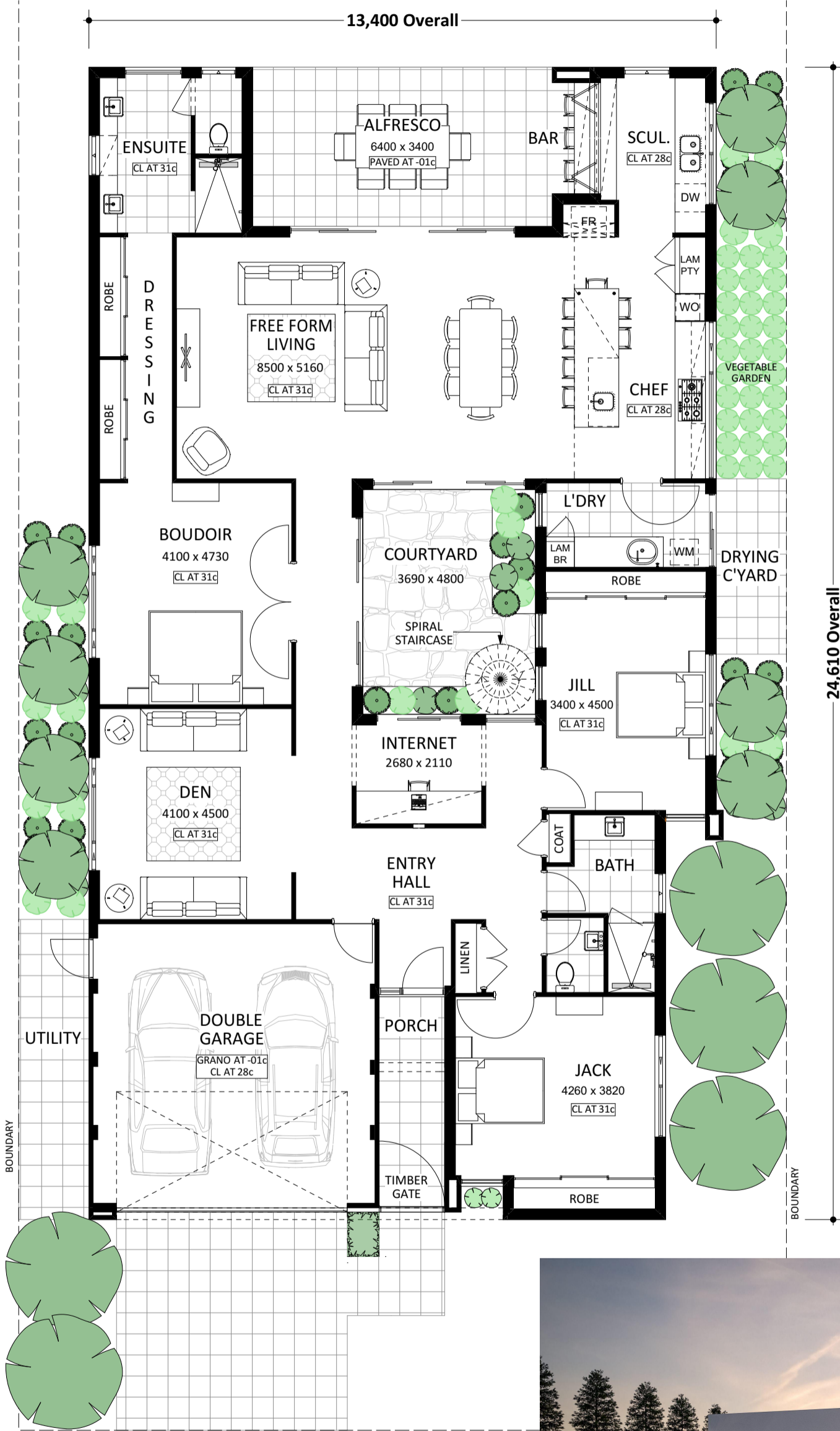
GROUND FLOOR PLAN 1:100
