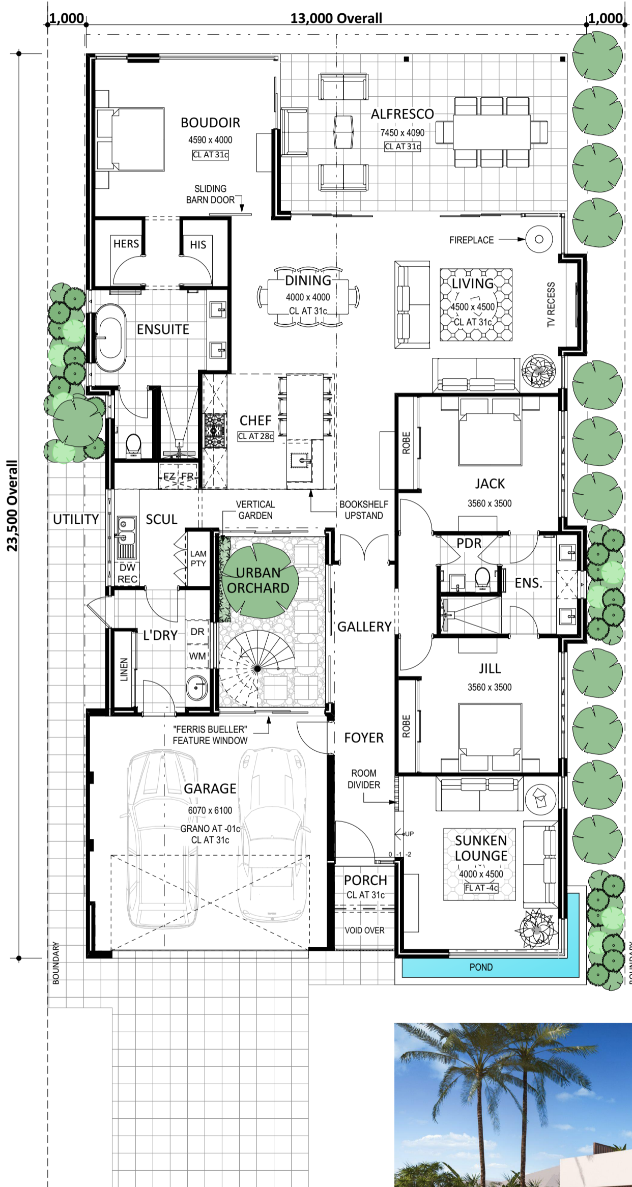
FLOOR PLAN 1:100
