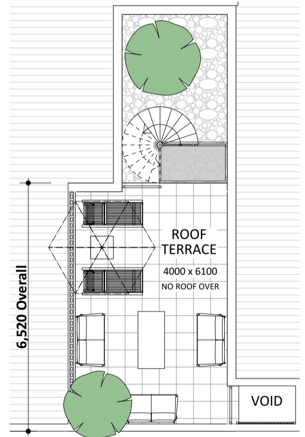
ROOF TERRACE 1:100
